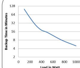
Runtime curve
