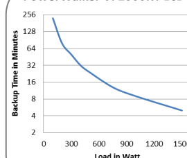
Runtime curve
